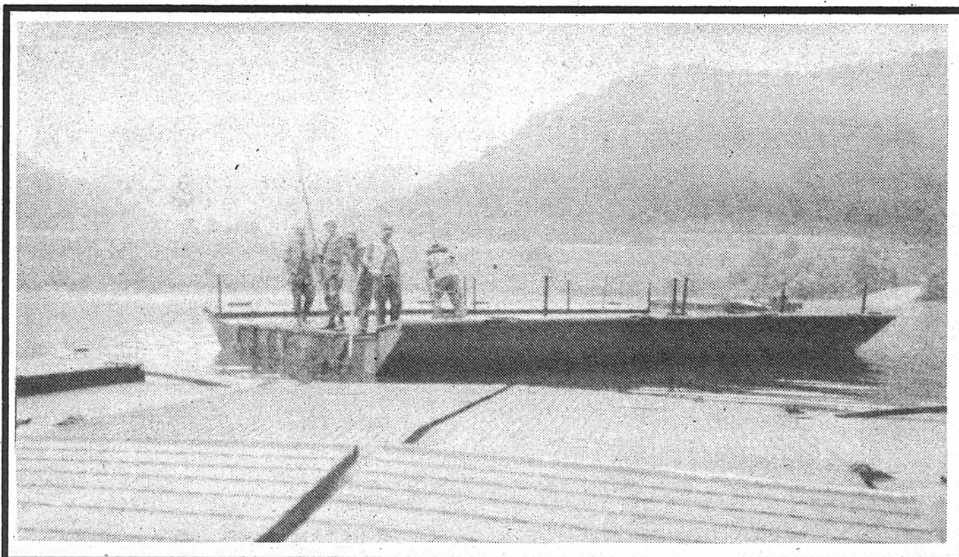
GETTING IT TOGETHER --Members of the Morehead unit of the Kentucky Army National Guard lash "bays" of a floating "ribbon" bridge to form a single span during a recent demonstration at Cave Run Lake near Morehead. Company E, 206th Engineer Battalion, is the only such unit in the state and among few of its type in the entire nation. It is part of the 35th Infantry Division (Mechanized). (Photo by SSG Steve Wright)
